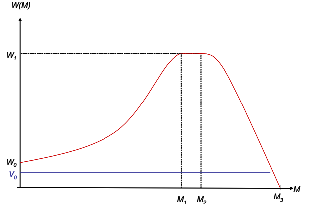
Eq. 3: No migration.
