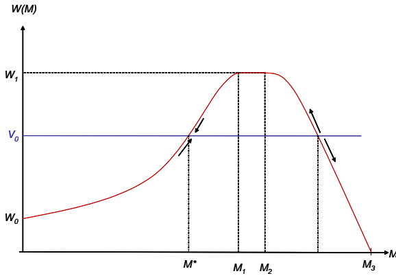
Eq. 2: Two steady equilibria.
