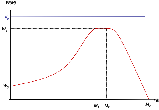
Eq. 0: Total migration.
