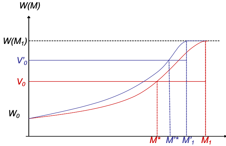
Figure 3: Impact of an increase of the net migratory benefit.
