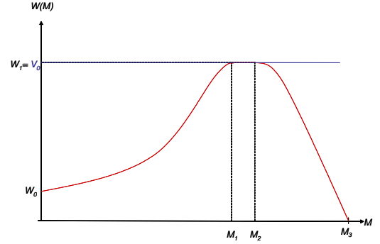
Eq. 1: Equilibria between M_1 and M_2 .
