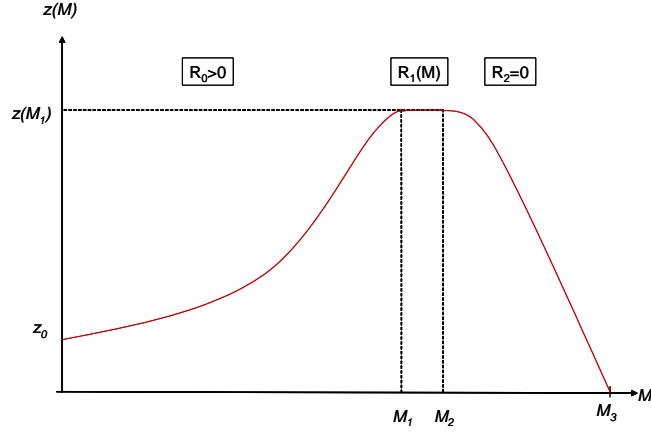
Figure 1: The income in the developing country.
