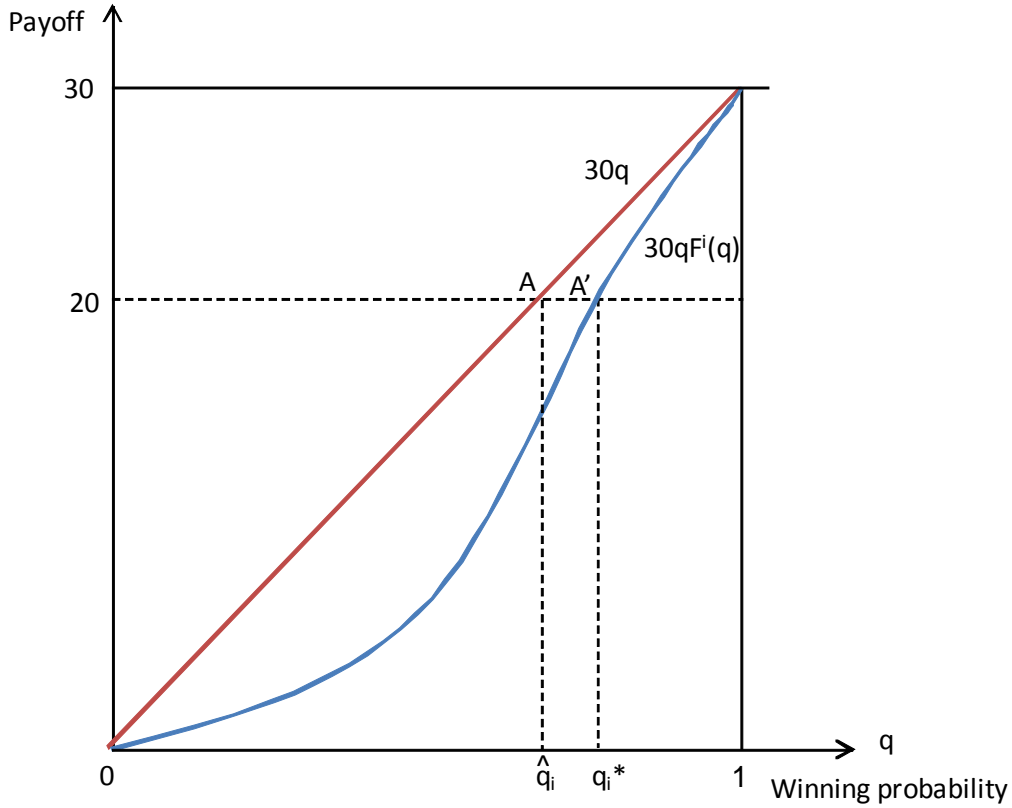
Figure 5: Critical winning thresholds for individual i
