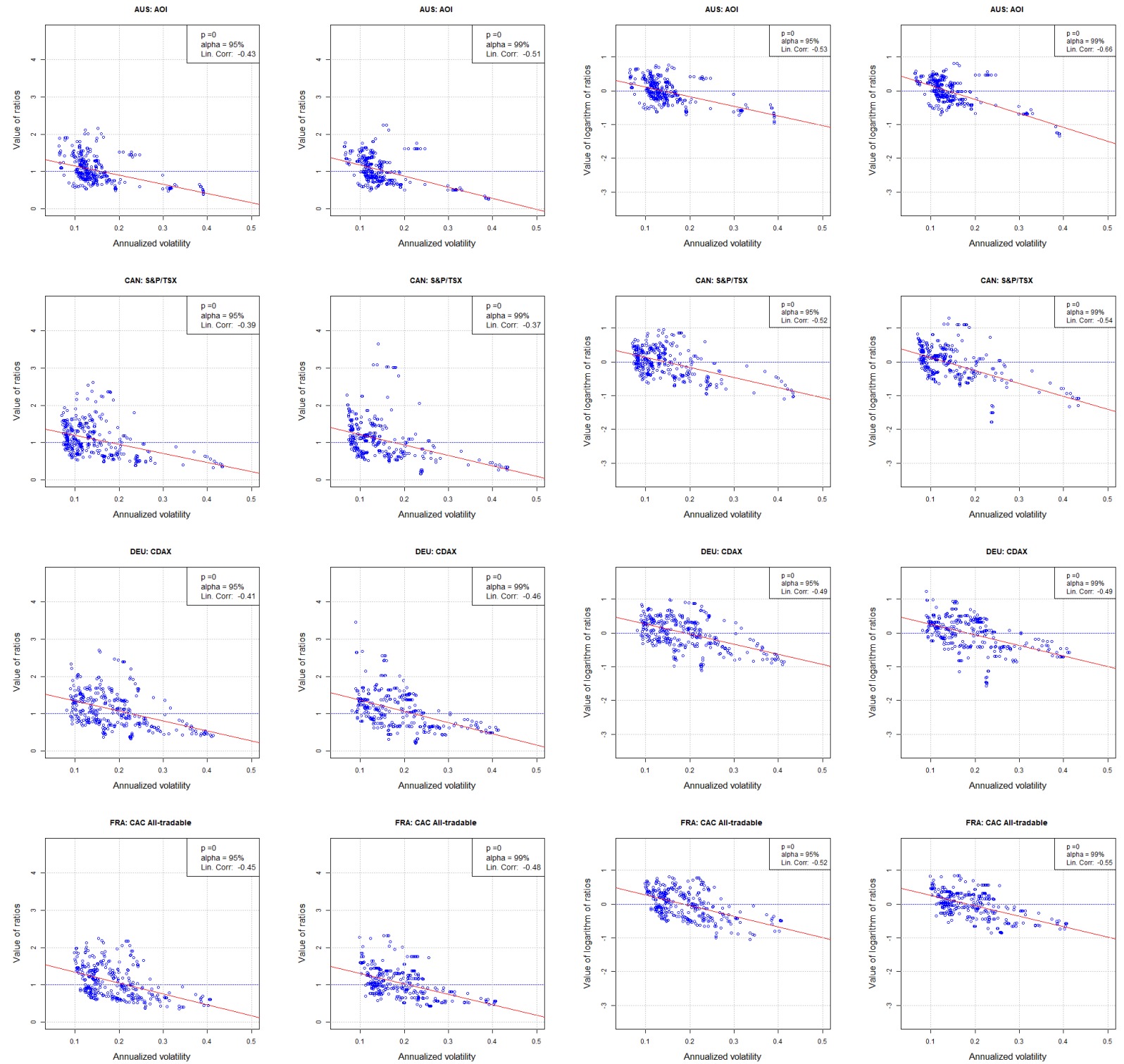
Figure A.9: SQP Ratios as a function of annualized volatility for p = 0 for \alpha = 95\% , 99\% . In each row we consider the SQP Ratios and then the logarithm of the SQP Ratios: From left to right, SQP ratio for \alpha = 95\% , 99\% , then logarithm of SQP ratio for \alpha = 95\% , 99\% . From top to bottom: AUS, CAN, DEU, FRA.
