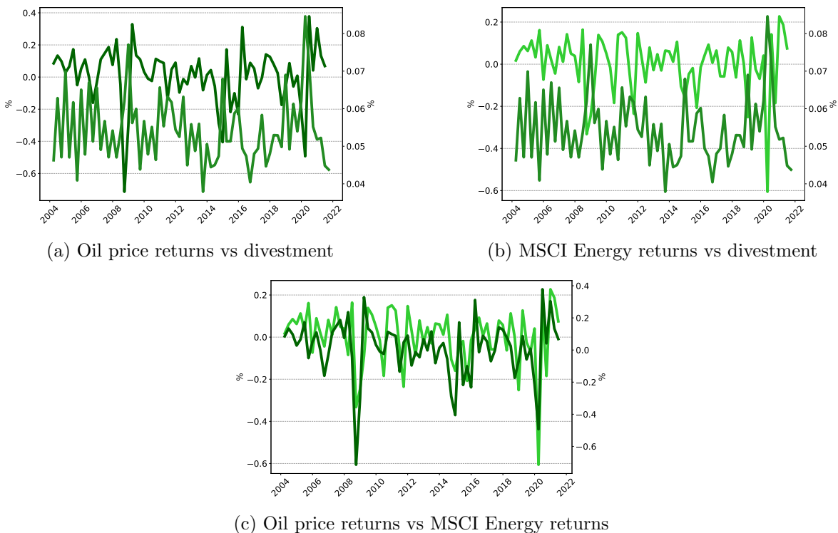
Figure 6: Variables co-movements
